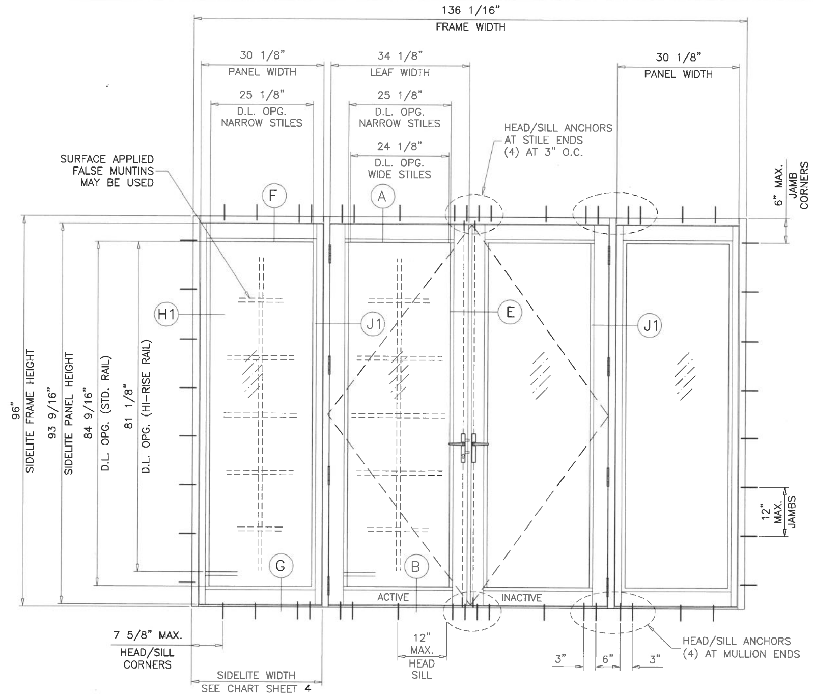
TYPICAL ELEVATION ( O-XX-O )
